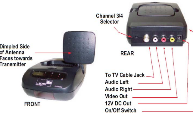
(B) Above photo Basic Receiver
